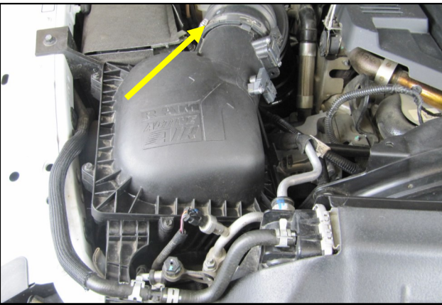
3. Loosen the clamp on the intake tube and remove the airbox lid from the vehicle.
